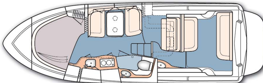
Cabin/Cockpit Layout w/Salon/Dinette (Plan A)
