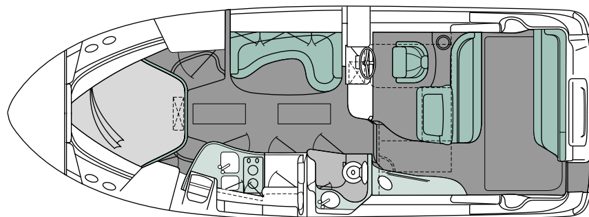
Cabin/Cockpit Layout
