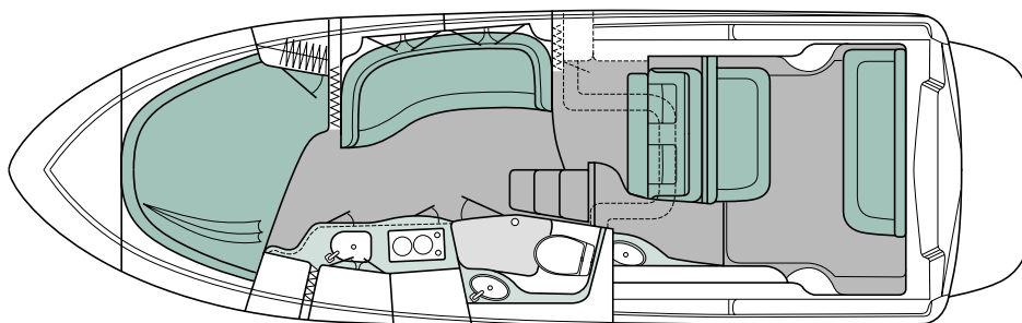
Cabin/Cockpit Layout w/Salon/Dinette (Plan B)
